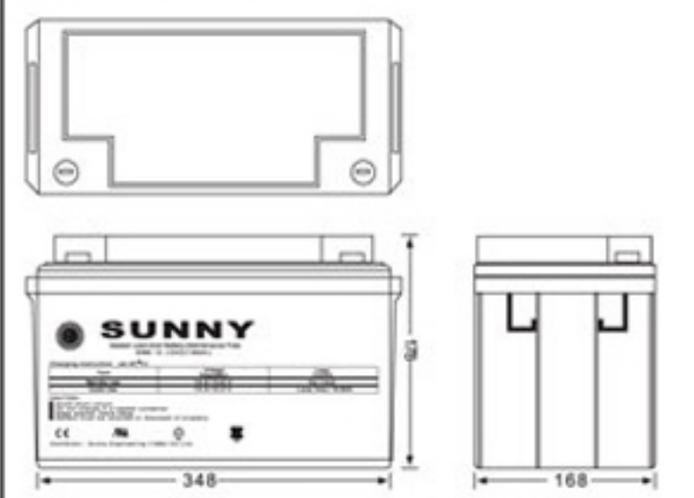
Dimensions(mm)
