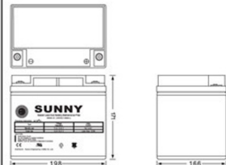
Dimensions(mm)
