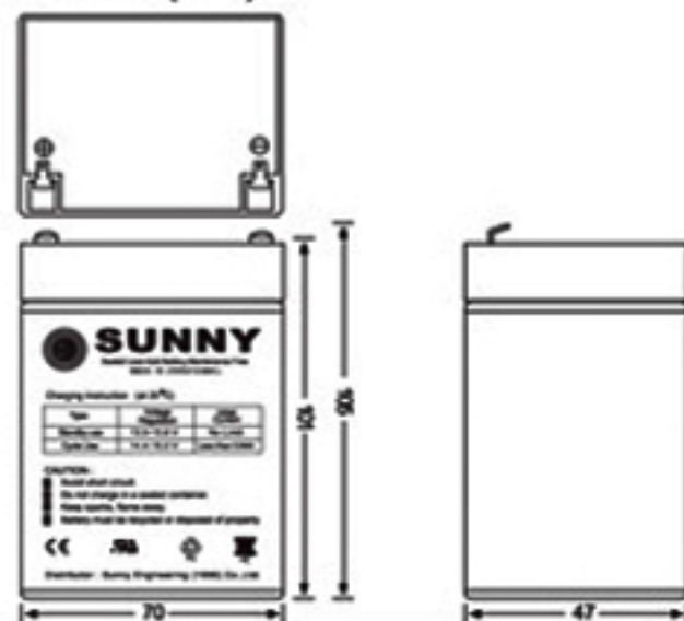
Dimensions (mm)
