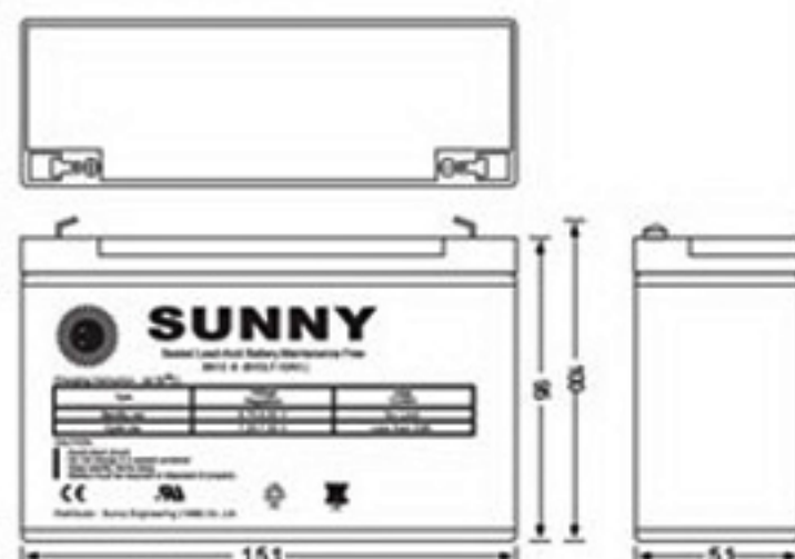
Dimensions(mm)
