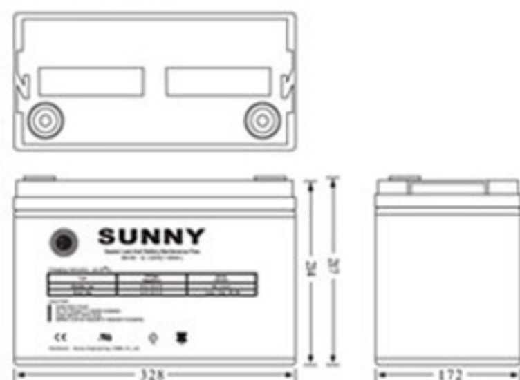
Dimensions(mm)
