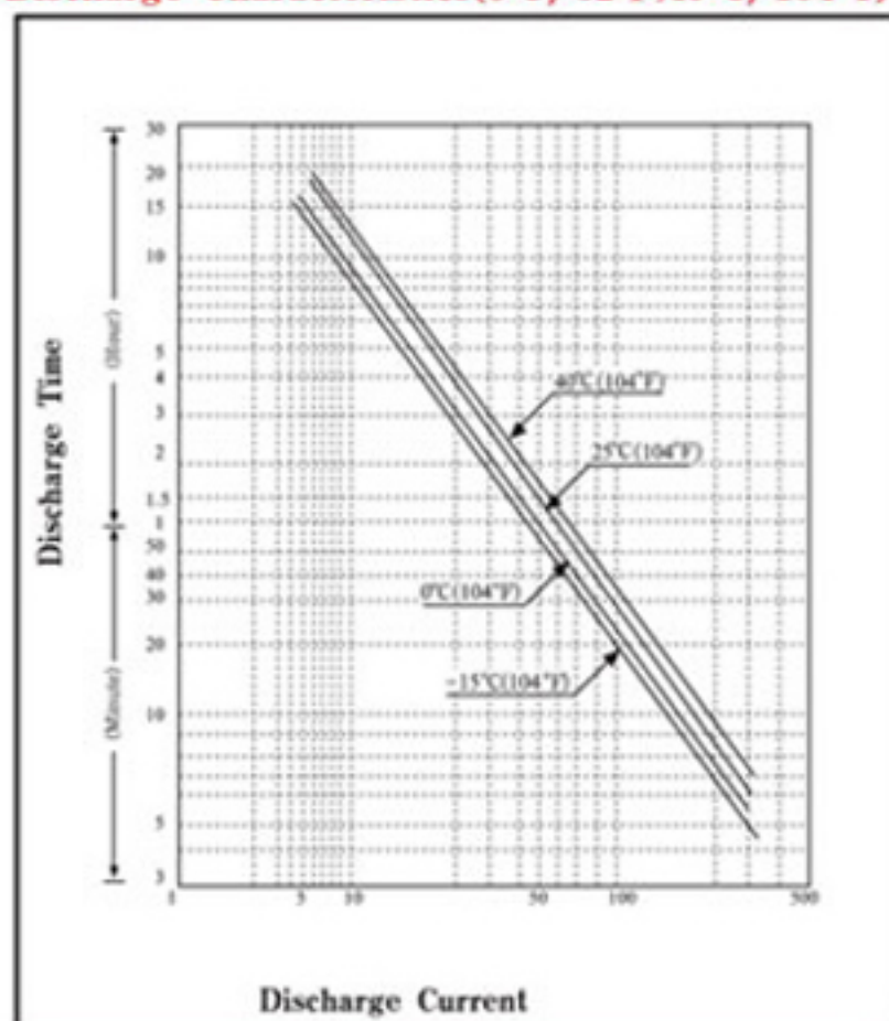
Discharge Characteristics(0°C/32°F,40°C/104°F)
