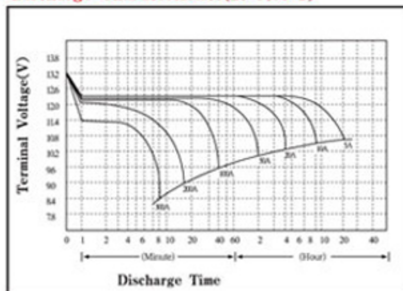
Discharge Characteristics(20°C,68°F)
